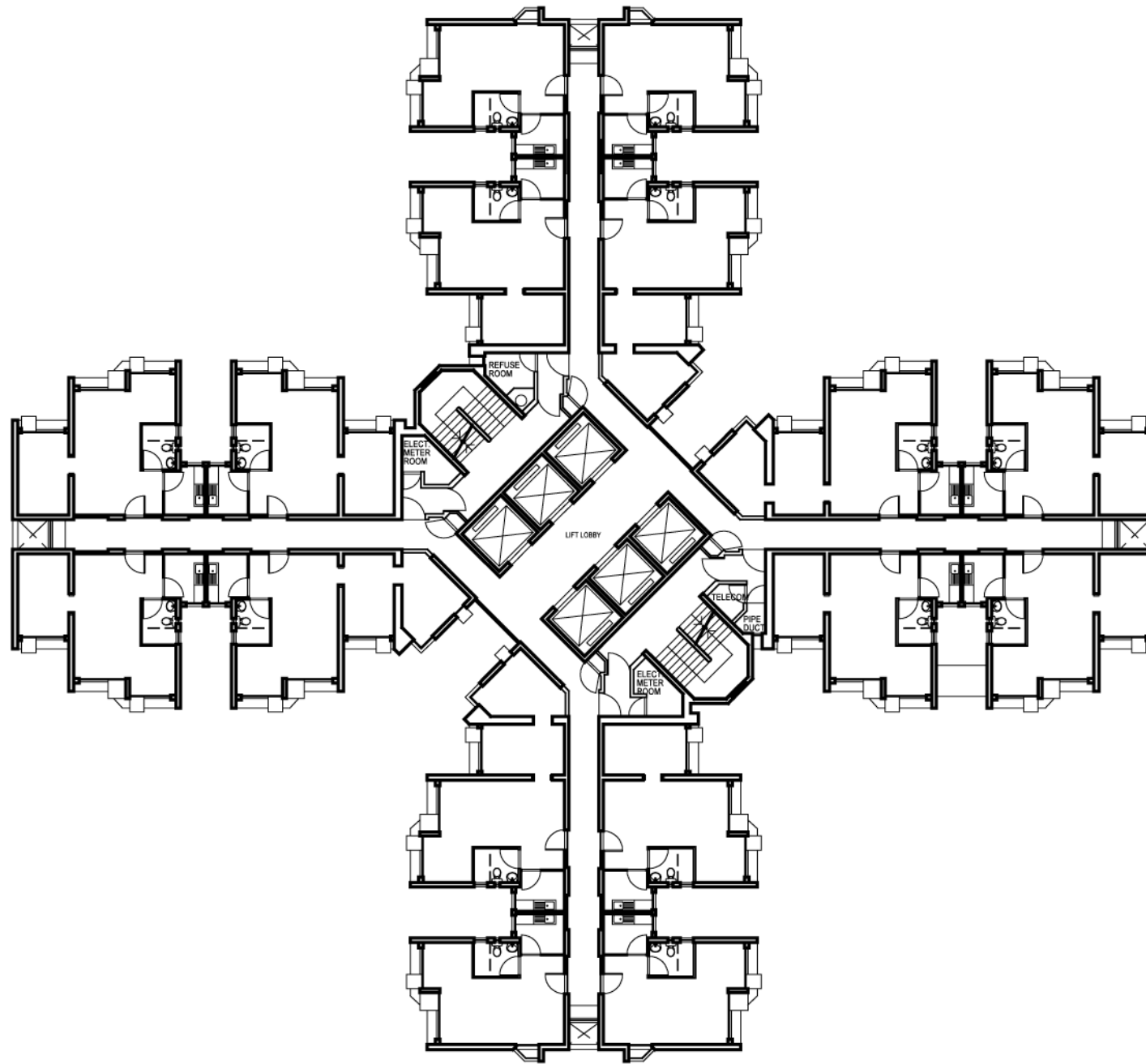
STANDARD BLOCK NEW HARMONY 1 (OPTION 4) TYPICAL FLOOR PLAN
