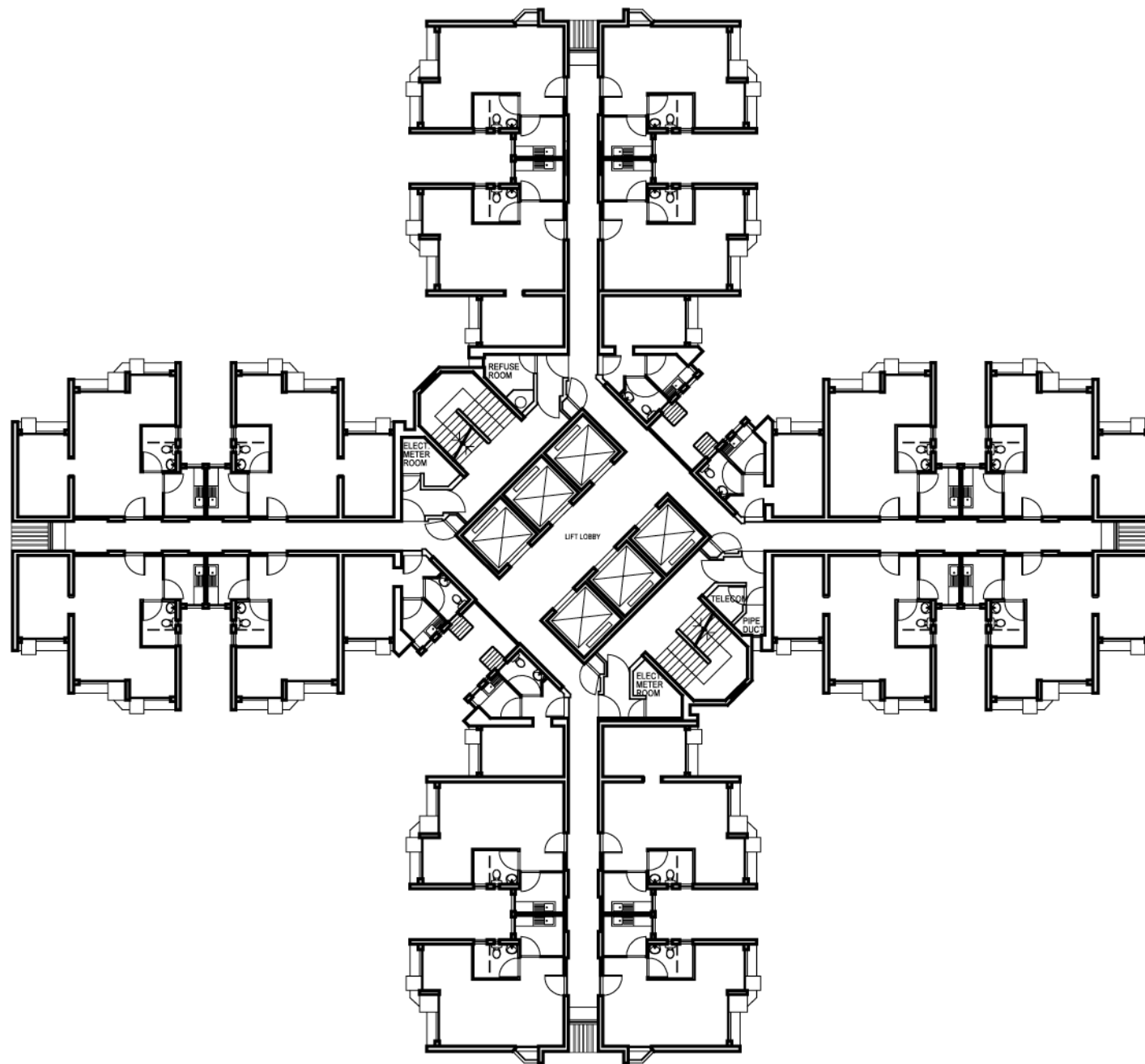
STANDARD BLOCK NEW HARMONY 1 (OPTION 3) TYPICAL FLOOR PLAN
